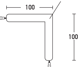
T24JA | TAF24 JOINT 90° | Ø24 x 100 x 100mm
