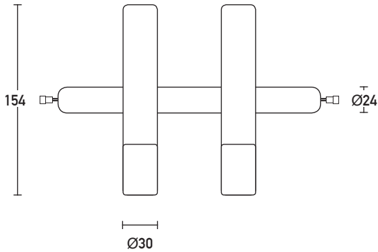
Segment | T24I31 | Ø30mm
