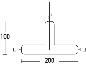
T24JT | TAF24 JOINT 'T' SHARE | Ø24
