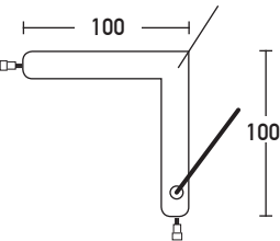
T24JF | TAF24 JOINT WITH FEEDER 90° | Ø24 x 100 x 100mm
